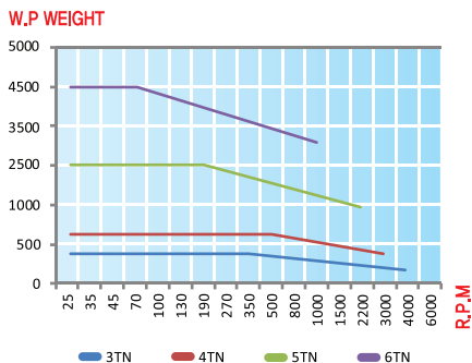
TN type technical data
