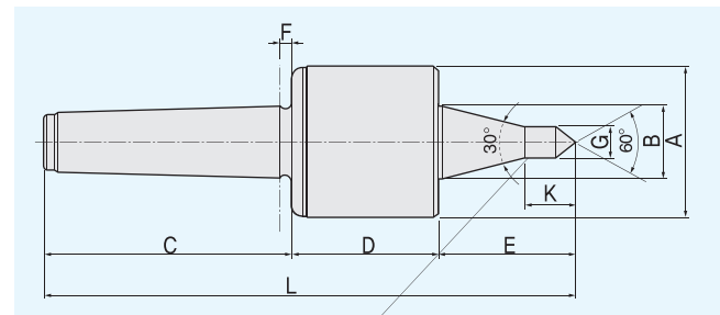
Elongated center point is specially shaped for improved tool clearance(Diagram)
