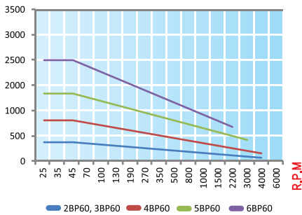
BP60 type technical data
